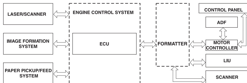
Figure 4-1. Product configuration
