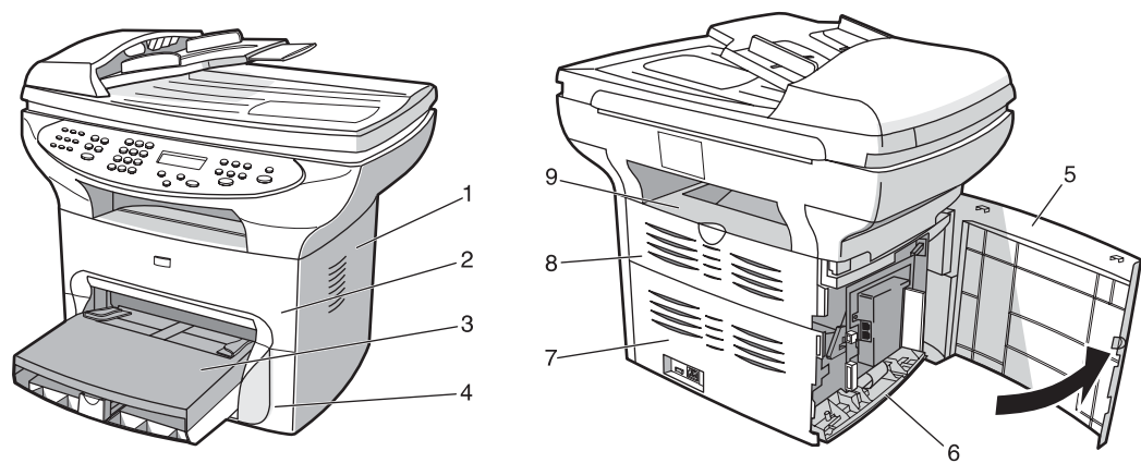
Figure 7-5. External components
