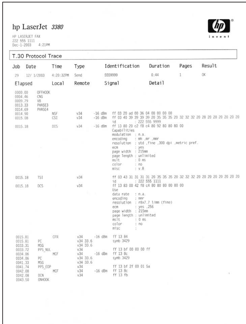
Figure 6-10. Example of a T.30 trace of a successfully sent fax
